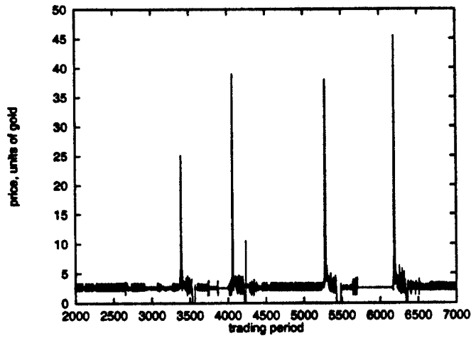
Fig 1. Market price history in a simulation with jumpy traders, illustrating bubbles and crashes.
