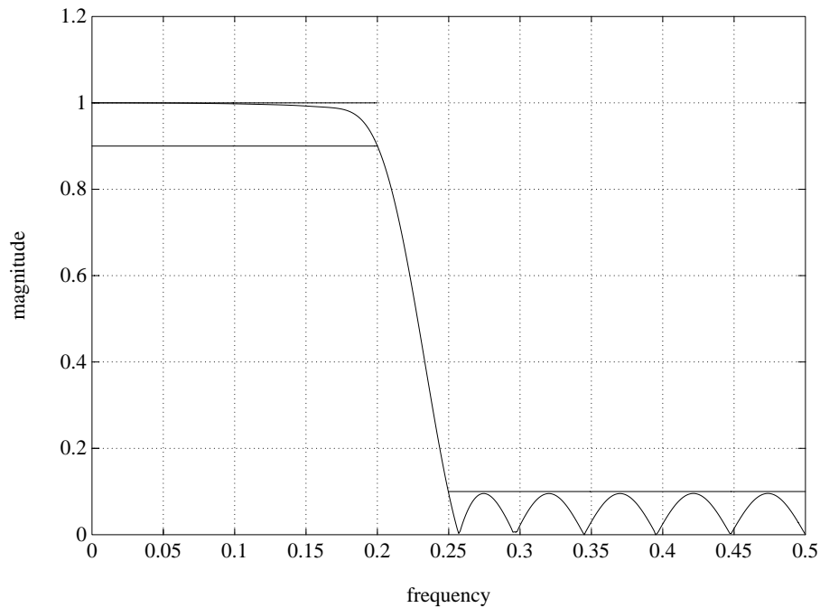
Figure 3. Flat Passband, Length-22, Minimum-Phase Filter.
