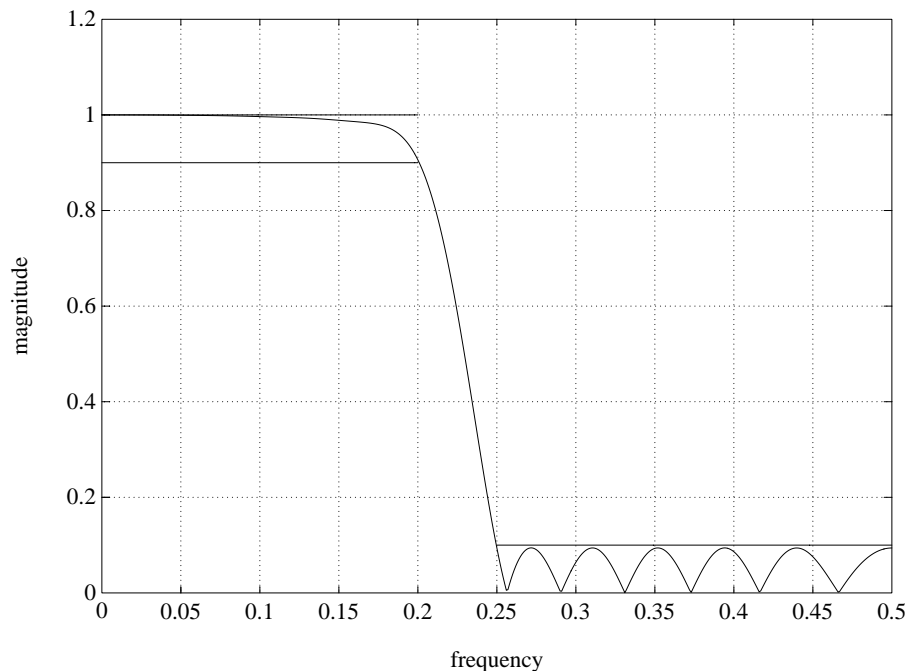
Figure 2. Length-29 Filter with Monotonically Decreasing Passband Response .
