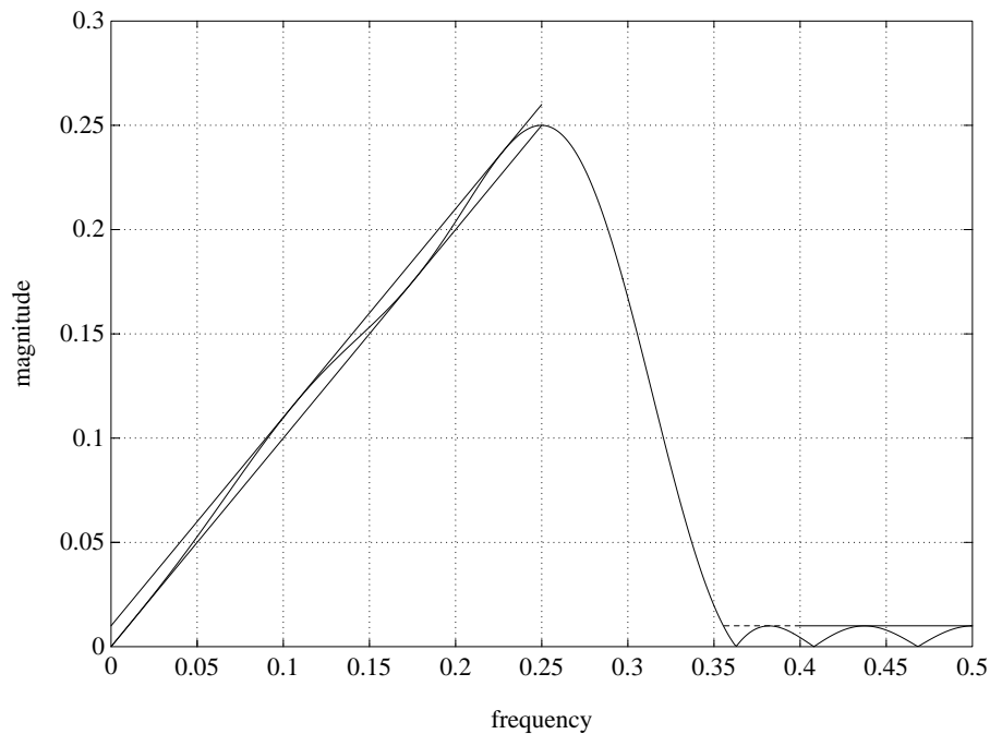
Figure 5. Frequency Response for Example 5, a Length-16 Lowpass Differentiator with a Minimum-Width Transition Band.
