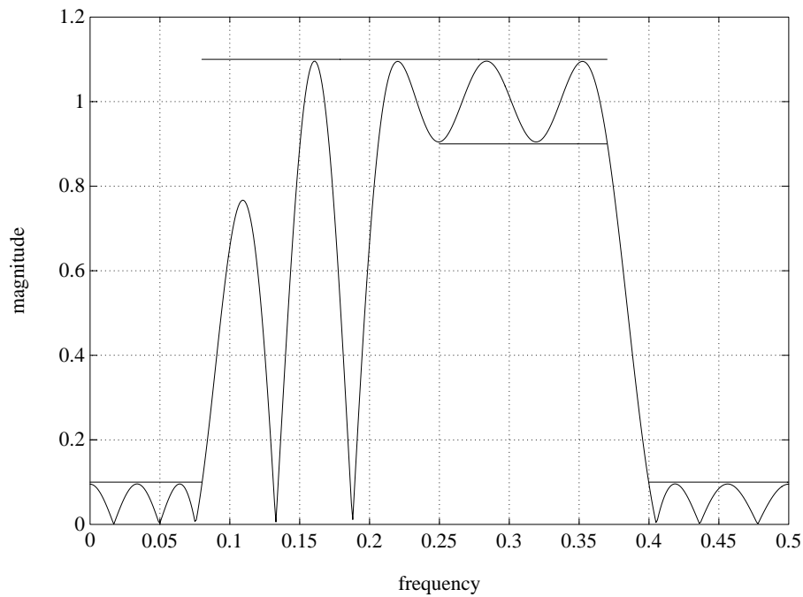
Figure 7. Length-27 Bandpass Filter with Transition Limits.
