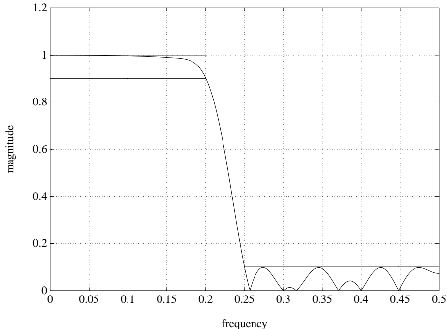
Figure 4. Length-29 Filter with Point Constraints .
