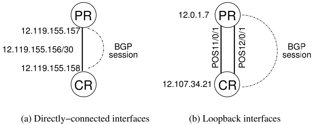
Figure 2: Two ways to reach the Customer Router's end of the BGP session
