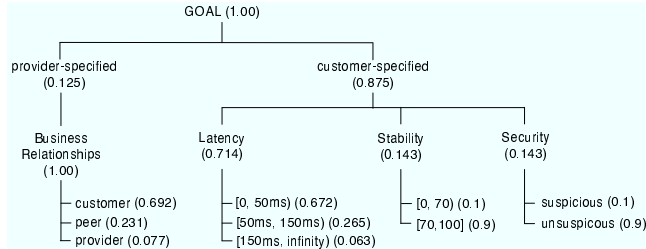
Fig. 7. The AHP hierarchy of an example routing policy
