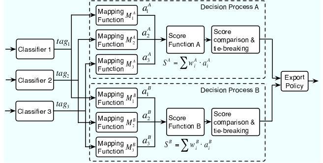
Fig. 4. Each decision process consists of a set of mapping functions of the policy objectives and a score function. Different decision processes are configured with different mapping functions and/or score functions to realize different policies.
