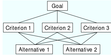
Fig. 5. The decision hierarchy of AHP.
