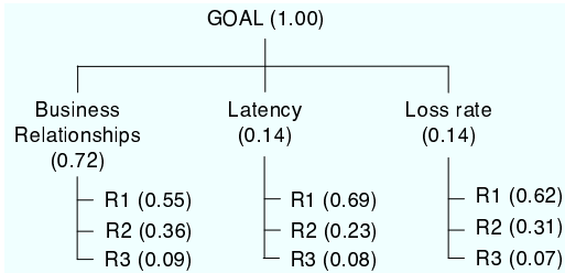
Fig. 6. Example of a decision hierarchy.
