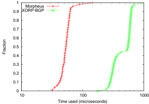
Fig. 9. Decision time: comparison between Morpheus and XORP-BGP (20 routes per prefix)
