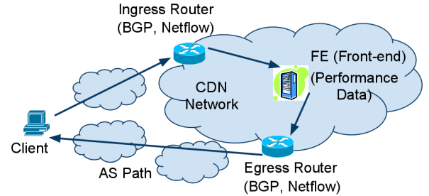
Fig. 1. CDN architecture and measurements
