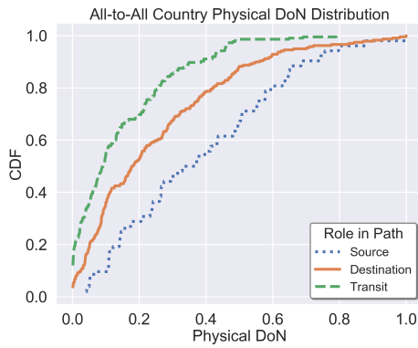
Figure 10: All-to-All Distribution of Physical DoNs
