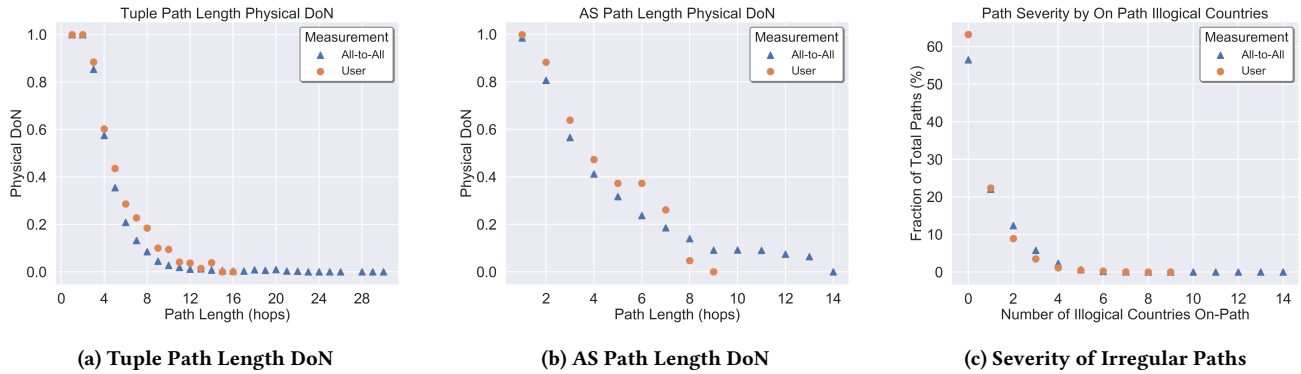
Figure 9: Examining the DoN through different lenses.
