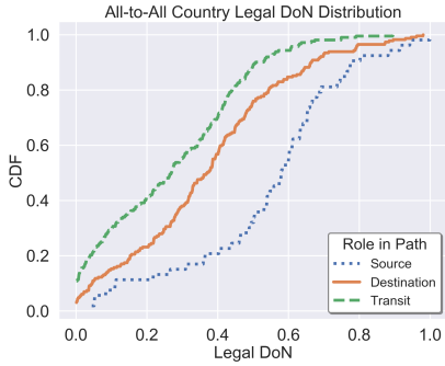
Figure 14: All-to-All Distribution of Legal Country DoNs
