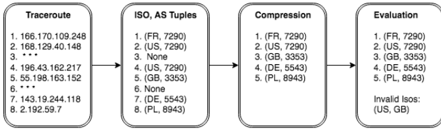
Figure 4: The process of transforming and formulating a traceroute based on its geographically (il)logical state.
