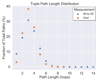
Figure 7: From a AS, Country tuple standpoint, the All-to-All paths are longer than the User study.
