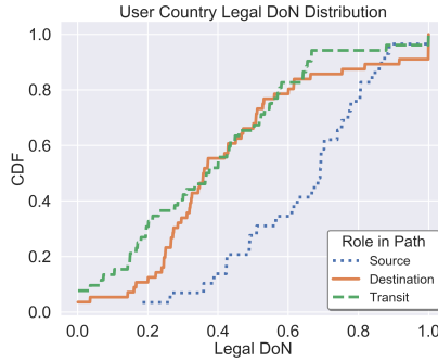
Figure 15: User Distribution of Legal Country DoNs
