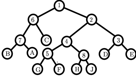
(b) Binary space partition
