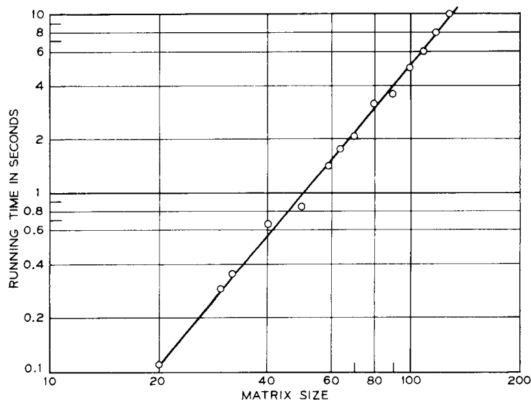
Fig. 2 — Running time.
