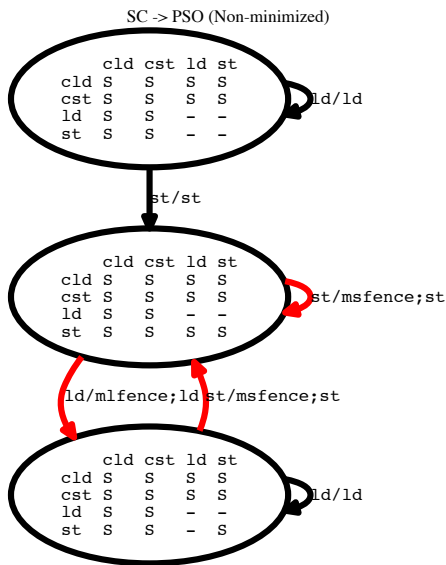
Figure A.6.c: FSM (Pre-minimization)
