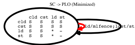
Figure A.5.d: FSM
