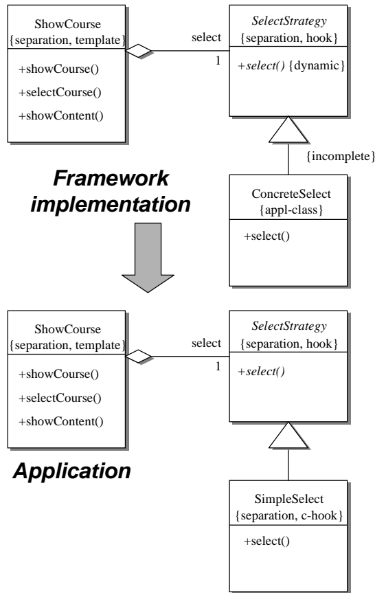
Figure 7. Instantiation example.
