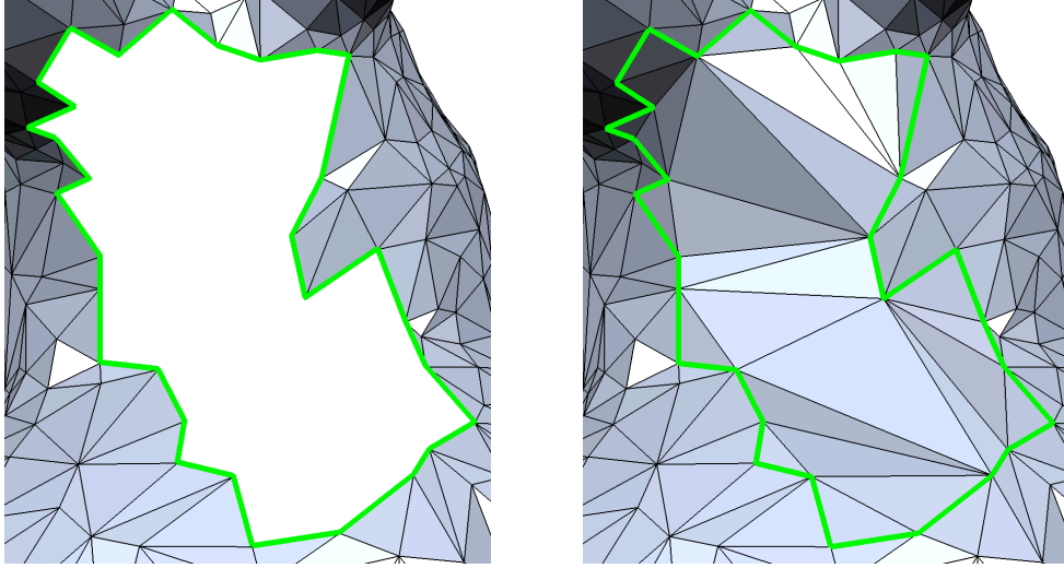
Figure 4.2: A hole triangulation that minimizes normal variation and total area.
