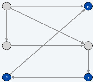
{ v, w, x } is feasible
