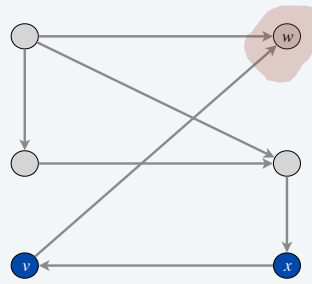
{ v, x } is infeasible
