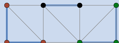
graph G
