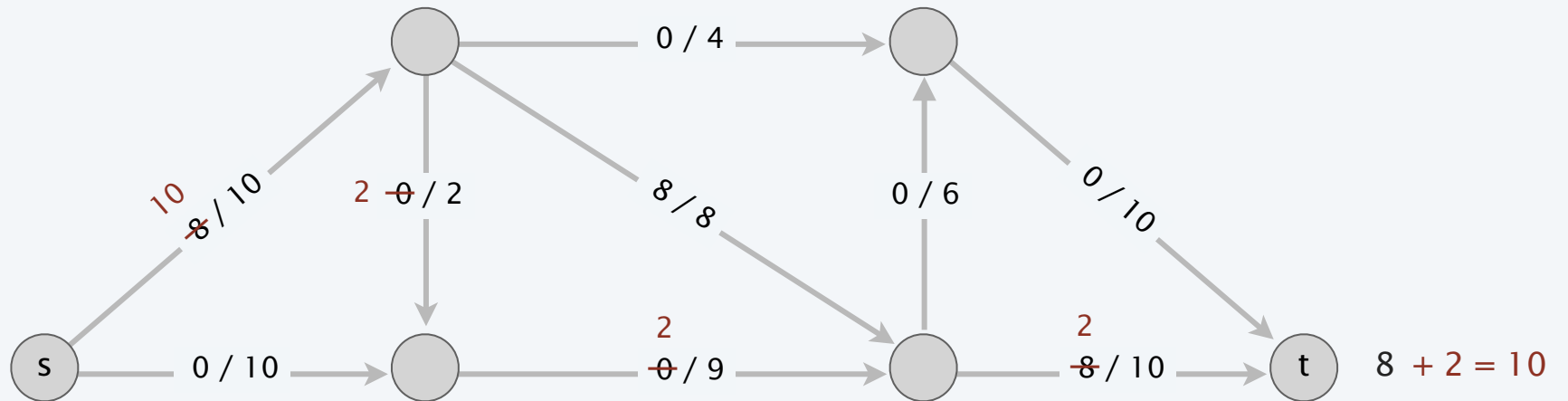
network G
