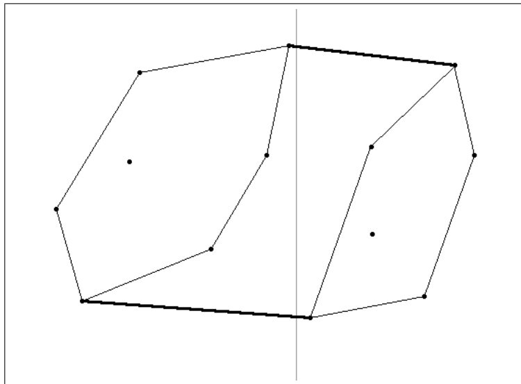
Step 1: Compute the convex hull for the left and right set of points
