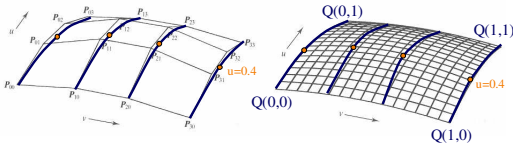
Watt Figure 6.21
