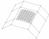
Watt Figure 6.28
