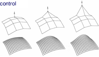
Watt Figure 6.22
