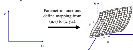
FvDFH Figure 11.42
