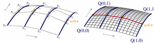
Watt Figure 6.21
