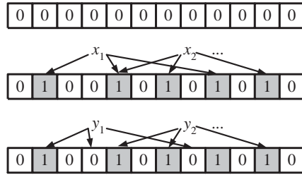
Figure 1: An example of a Bloom filter. The filter begins as an array of all 0's. Each item in the set x_i is hashed k times, with each hash yielding a bit location; these bits are set to 1. To check if an element y is in the set, hash it k times and check the corresponding bits. The element y_1 cannot be in the set, since a 0 is found at one of the bits. The element y_2 is either in the set or it has yielded a false positive.
