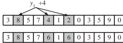
Figure 2: An example of conservative update. This flow can only have been responsible for 2 previous bytes, so when it introduces 4 new bytes, counters should increase only to 6.
