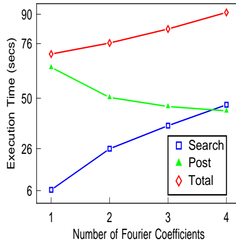
Figure 4: Breakup of the execution time, for all-pairs query ( |\mathcal{S}| = 400 )
