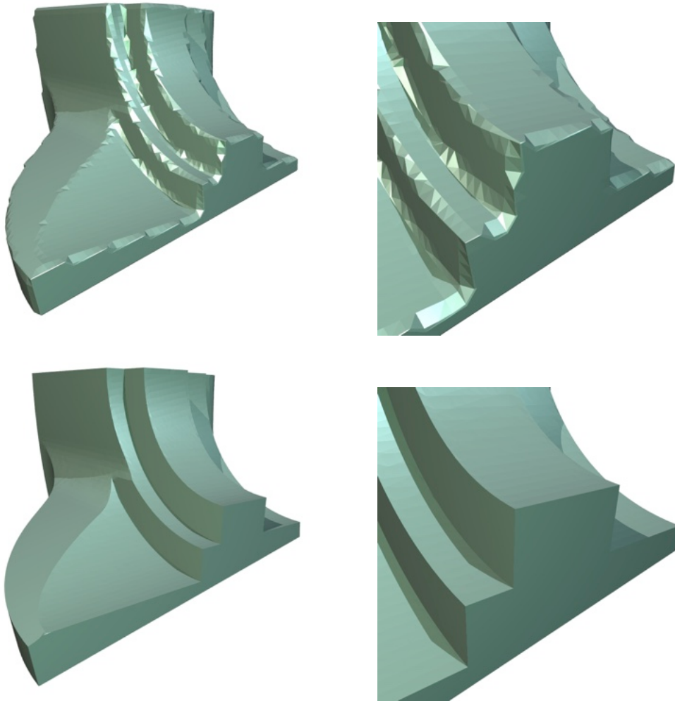
Figure 2.10: Two reconstructions of the “fandisk” dataset from a 65 \times 65 \times 65 sampling of its signed distance field. The standard Marching Cubes algorithm leads to severe alias artifacts near sharp features ( top ), whereas the feature-sensitive iso-surface extraction faithfully reconstructs them ( bottom ).
