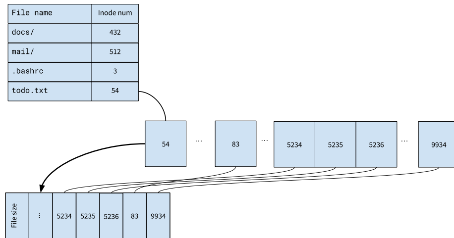
Figure 4: A directory is a special type of file that maps filenames to inode numbers
