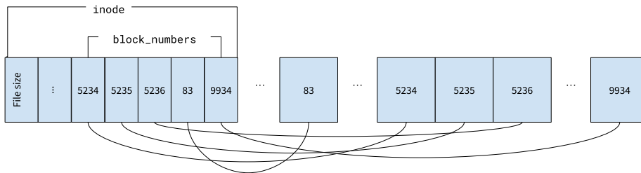
Figure 3: The inode struct is store in a block and points to blocks containing file data
