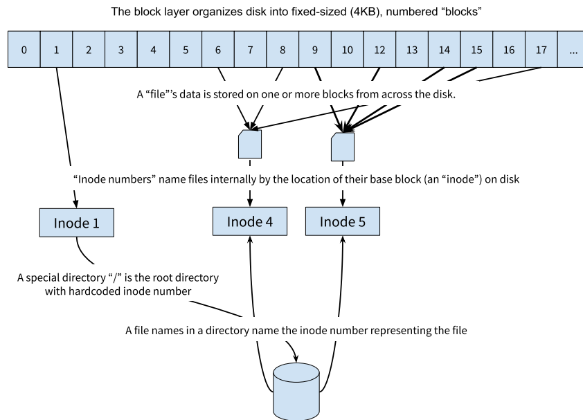
Figure 1: The UNIX File System's Naming Hierarchy
