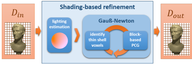
Figure 4: At each hierarchy level, lighting is estimated based on the fused model and the spatially-varying albedo estimates. Then, albedos and geometry of voxels within a thin-shell are optimized.
