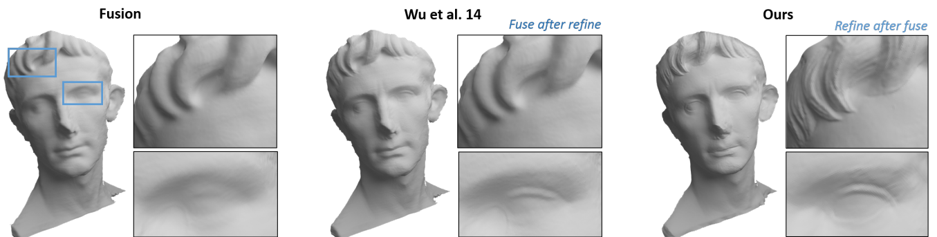
Figure 13: The method of Wu et al. [2014] refines independent depth maps, causing detail to smooth out in the subsequent fusion process; i.e., fuse after refine. Our method refines the geometry after surface fusion, i.e., refine after fuse, thus capturing substantially more detail.
