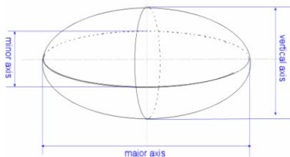
Figure 2: 3D-Ellipsoid and its axes
