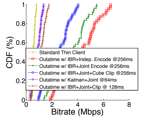
Figure 17: Bandwidth Overhead
