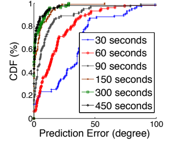
Figure 5: Error Decreases with More Observation Time. Data is for Fable 3 at RTT=160ms.
