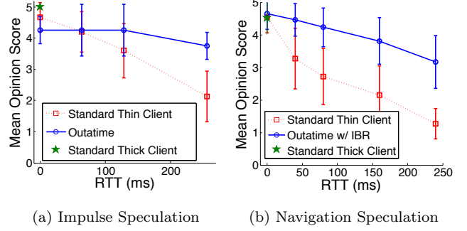
Figure 14: Table 3 MOS
