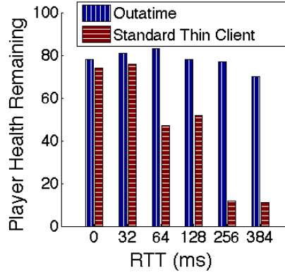
Figure 12: Remaining Health
