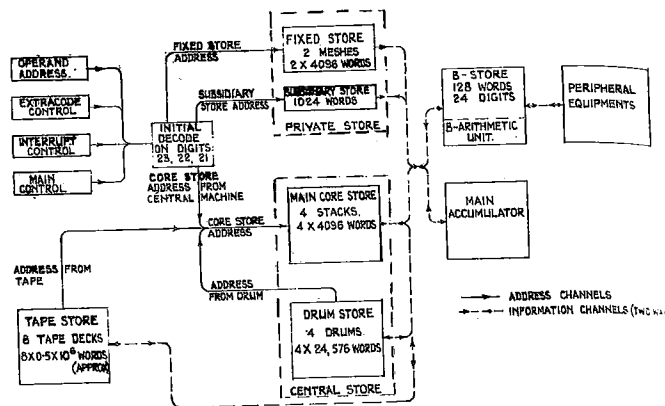
Fig. 1—Layout of basic machine.
