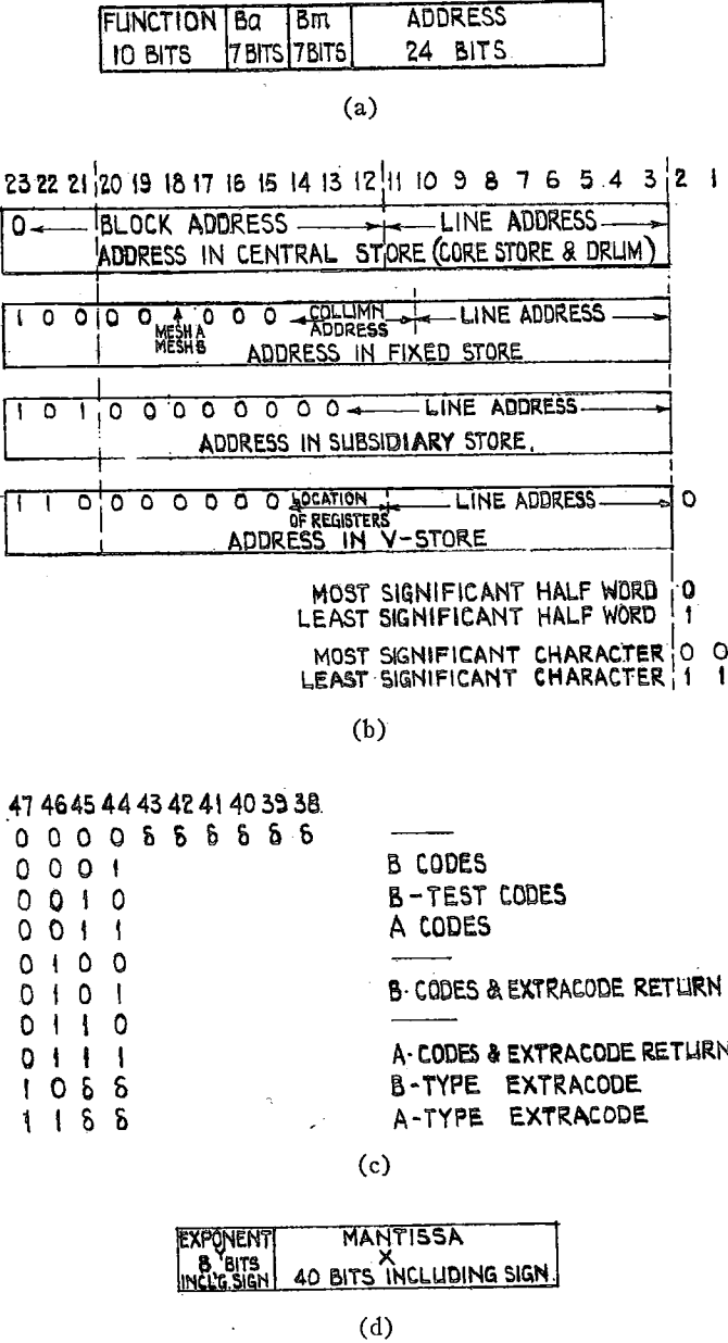
Fig. 2—Interpretation of a word. (a) Form of instruction. (b) Allocation of address digits. (c) Function of decoding. (d) Floating point number X8^E .
