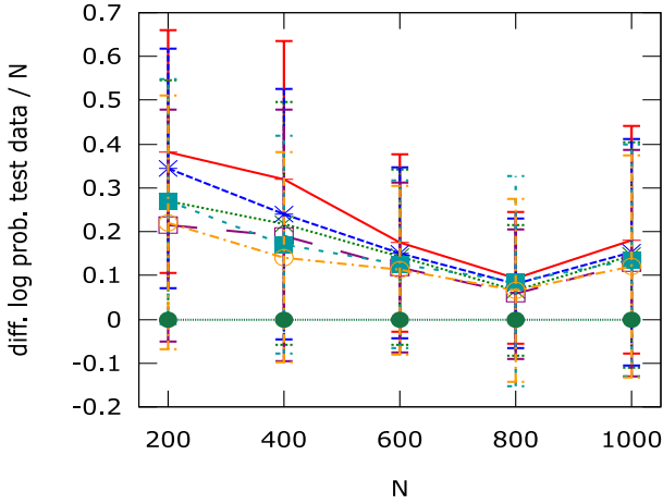
Figure 3: Relative average log probability per data-point for test data as a function of N .
