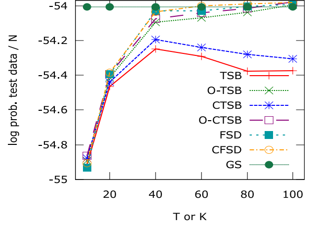
Figure 4: Average log probability per data-point for test data as a function of T (for TSB methods) or K (for FSD methods).
