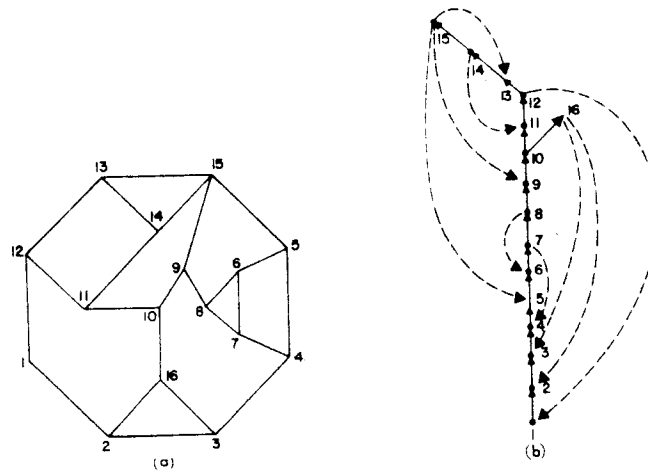
FIG. 3. (a) A graph G to be tested for planarity; (b) a palm tree P generated from G . Upward, solid edges are tree arcs. Downward, dotted edges are fronds. Vertices are numbered in search order.
