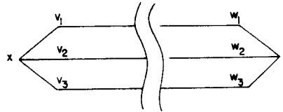
FIG. 2. Illustration of Lemma 2. Path p_2 is inside the simple closed curve formed by p_1 and p_3 .
