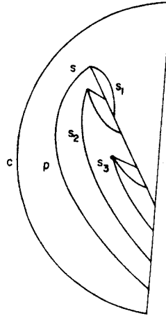
Fig. 7. Recursive application of the embedding algorithm. Segment S consists of first path p and new segments S_1, S_2, S_3 .
