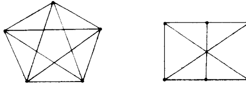
FIG. 1. The Kuratowski subgraphs
