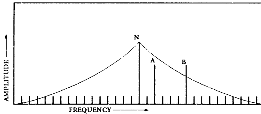
Figure 3.20: Critical-Band Masking
