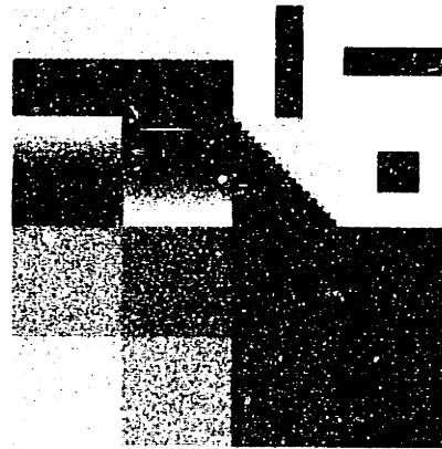
Figure 3.8: Test Image
