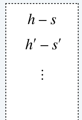
stable matching M
