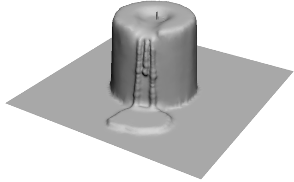
Figure 9. Compared to the melting candle modeled with a level set approach (Figure 5), this example demonstrates the fine resolution that meshes can provide while maintaining interactive simulation rates.
