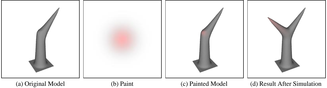
Figure 2. (a) In our system the user begins with a base model. In this example, it is the extended trunk of a stylized tree for a cemetery scene. (b) Next, the user selects the paint that will give the surface a desired type of deformation and a brush to modulate its intensity. Here the user has selected a paint-brush pair whose resulting motion will form a spiky protrusion. The paint creates positive speed of the surface (with respect to the surface normal) and is visualized in bright red. (c) Next, the user directly paints the surface of the model where they desire the simulated motion to occur. (d) Lastly, the user interactively simulates the motion of the surface until the final result is achieved. In this case, the user simulated the surface’s motion until the model included a branch of the desired length. Notice how the paint has moved with the surface during the physical simulation.
