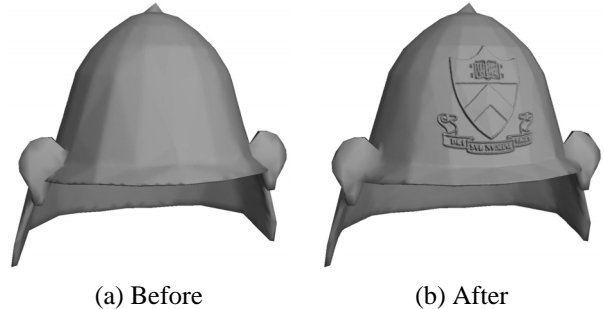
Figure 4. Simulating advective motion where the direction of the velocity is the existing surface normal can create embossing effects. In this example, the user adds the Princeton emblem to a kabuto by painting positive advective paint onto its crown.
