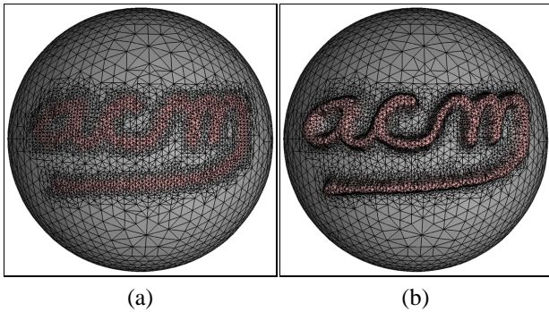
Figure 6. (a) We subdivide the mesh as a function of the painting direction and location. This refinement guarantees that vertices along the model’s surface accurately sample the brush bitmap. (b) This results in a mesh whose complexity matches the geometric detail of the deformation.
