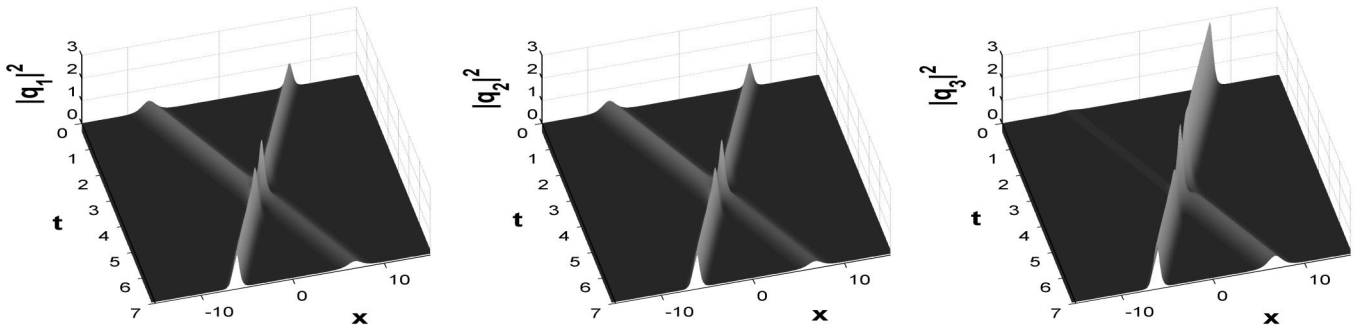
Figure 1: Collision of two 3-component solitons as described in the example. Shown are |q_1|^2 , |q_2|^2 , and |q_3|^2 , respectively. The scale is normalized. Each component of each soliton interacts with the same component of the other soliton (shown in the figure), and also with the intensity of the other two components (this interaction is not explicitly visible in the figure). Note the transfers of energy between solitons, especially pronounced in the third component.
