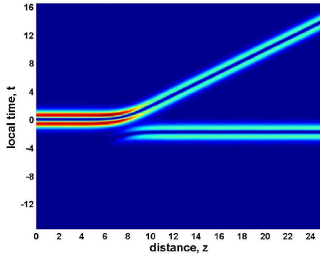
Figure 3: (Color online) The probe when launched in the state |21\rangle . In this case the soliton collision takes place at a greater relative velocity and the system acts as an ordinary non-polarizing beam-splitter. (See [3] for details.)
