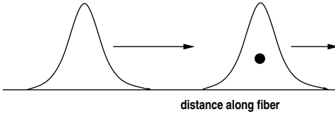
Figure 1: Sketch illustrating the conditions for photon transfer when a fast soliton overtakes a slower one.
