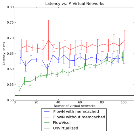
Figure 2: Latency vs. Virtual Network count
