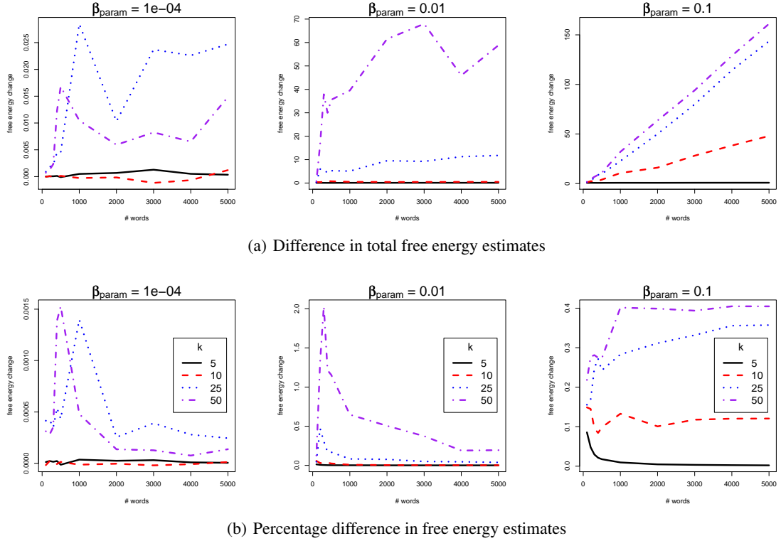
Figure 1: Results on synthetic text data. We sample k topics from a symmetric Dirichlet distribution with parameter \beta_{\text{param}} . We sample 10 documents from LDA models with these topics. We consider prefixes of varying lengths for each document. For each prefix length, the VB and CVB free energies are averaged over the 10 documents. The curves obtained show how the advantage of CVB over VB changes with the length of a document, number of topics and sparsity of topics.
