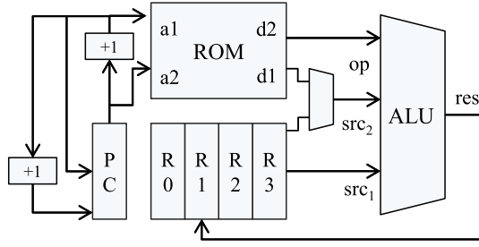
Fig. 3. Simple processor for illustration.
