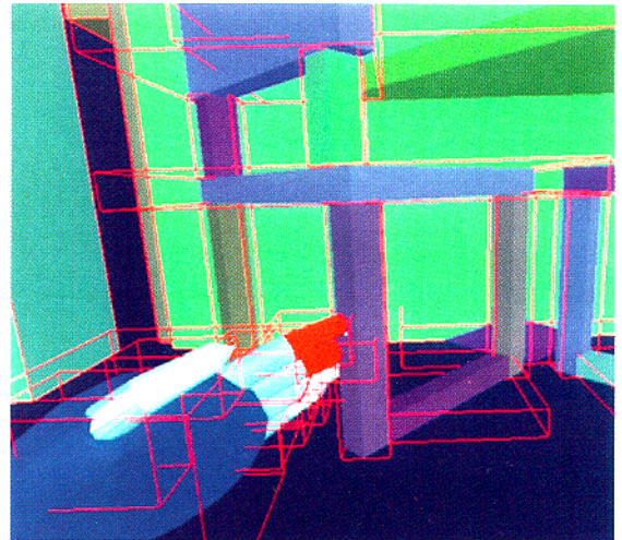
Frame 4: Red polytopes indicate collisions.
