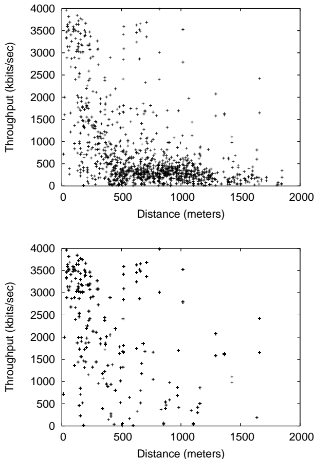
Figure 3: Link throughput versus distance for all links (top) and for the links used by Srcr (bottom). Srcr makes the most use of short high-throughput links. (single-hop TCP, multi-hop TCP)
