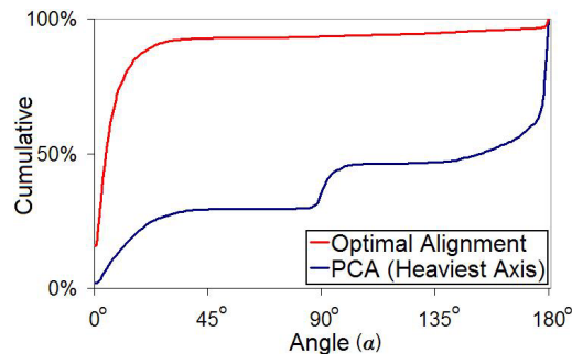
Figure 14: A plot showing the percentage of models aligned within a certain tolerance angle, \alpha (horizontal axis). The graph shows results for PCA alignment with heaviest axis flip and our optimal alignment. Note that for a small error tolerance (e.g., within 10^\circ ), the optimal alignment algorithm succeeds for a much greater percentage of the models.
