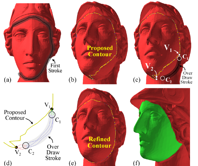
Figure 5: Cutting the face of Athena with intelligent scissoring: (a) the user draws an imprecise first stroke (gray); (b) the system proposes a cut (yellow curve); (c) the user draws an overdraw stroke (gray) to refine the cut; (d) the system splices in the least cost path traveling from V_1 first to C_1 (red) then to C_2 within the stroke (blue) and finally to V_2 (green); (e) the proposed cut contour is updated; (f) the final result is a segmentation of the mesh into two parts (green and red) separated by natural seams of the mesh.
