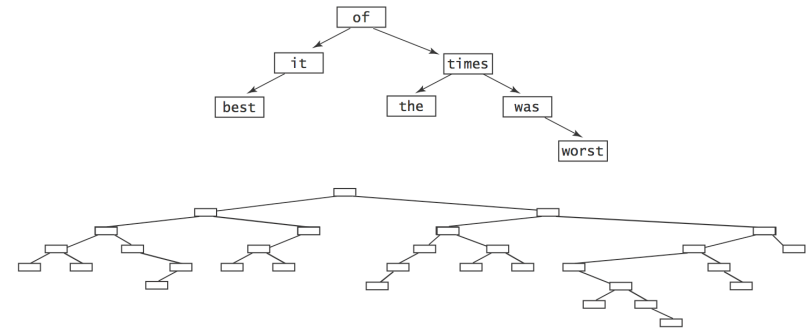
Typical BSTs constructed from randomly ordered keys
