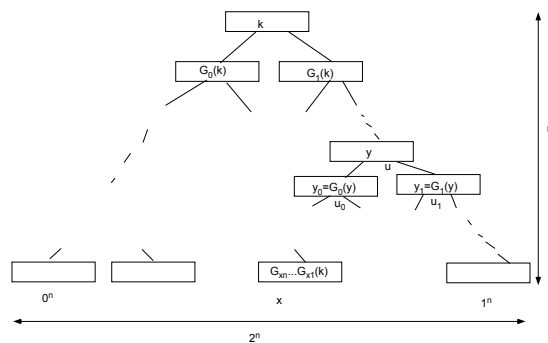
Figure 9.2: The pseudorandom function f_k(x) outputs the label of the x^{th} node in a depth n binary tree where the root is labeled by k , and the children u_0, u_1 of every node u labeled y are labeled by G_0(y) and G_1(y) .
