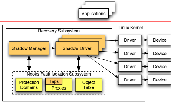
Figure 4: The Linux operating system with several device drivers and the driver recovery subsystem. New code components include the taps, the shadow manager and a set of shadow drivers, all built on top of the Nooks driver fault isolation subsystem.
