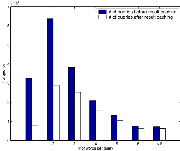
Figure 6.2: Number of queries before and after result caching.
