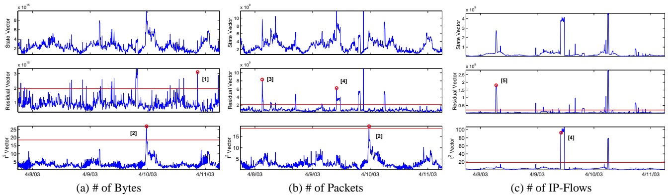
Figure 1: An illustration of the subspace method on the three types of OD flow traffic. Top row: timeseries of state vector squared magnitude ( \|\mathbf{x}\|^2 ); middle row: timeseries of the residual vector squared magnitude ( \|\hat{\mathbf{x}}\|^2 ); bottom row: t^2 vector.
