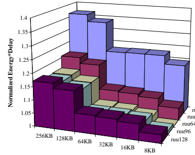
Figure 12: Energy-Delay Product for turb3d .
