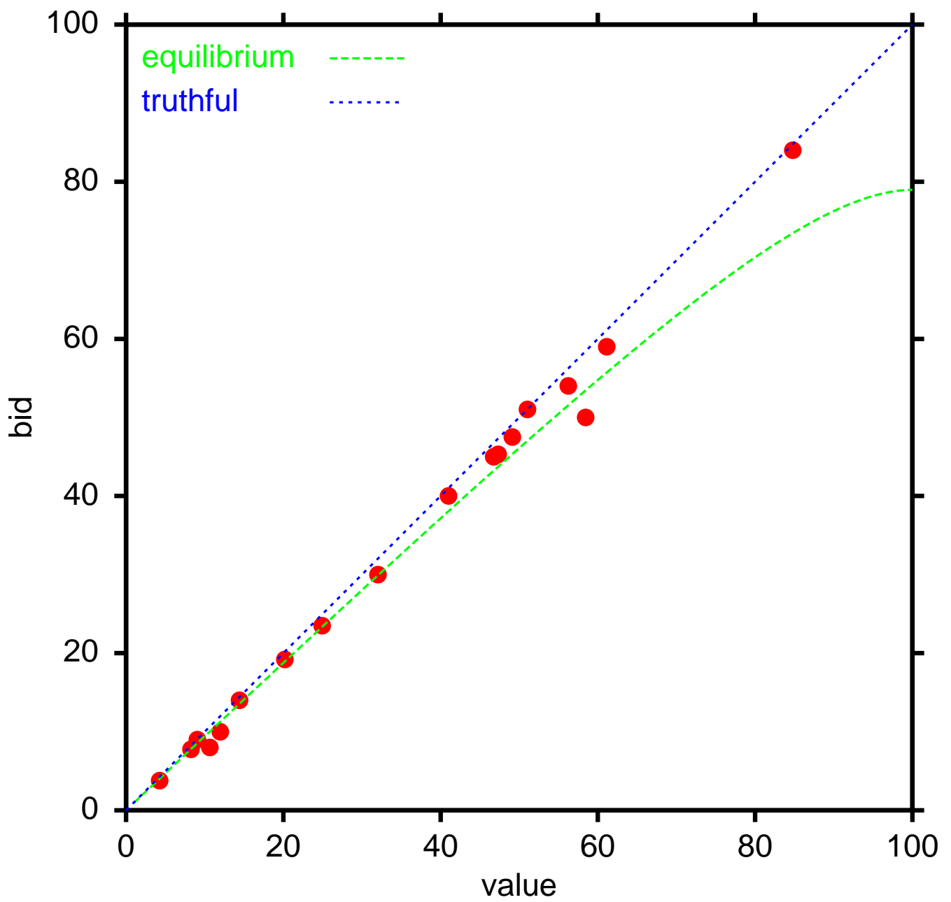
First-Price, density is linear downslope [0,$100], n=18
