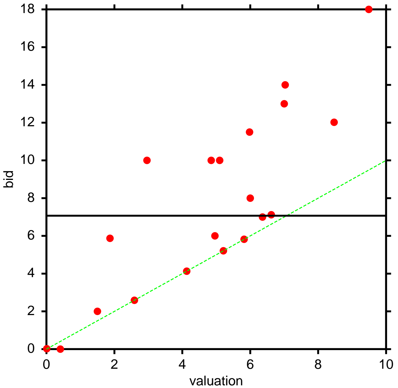
Average-of-others, no cap, v's iid on [0,$10], Feb. 19, 2009
