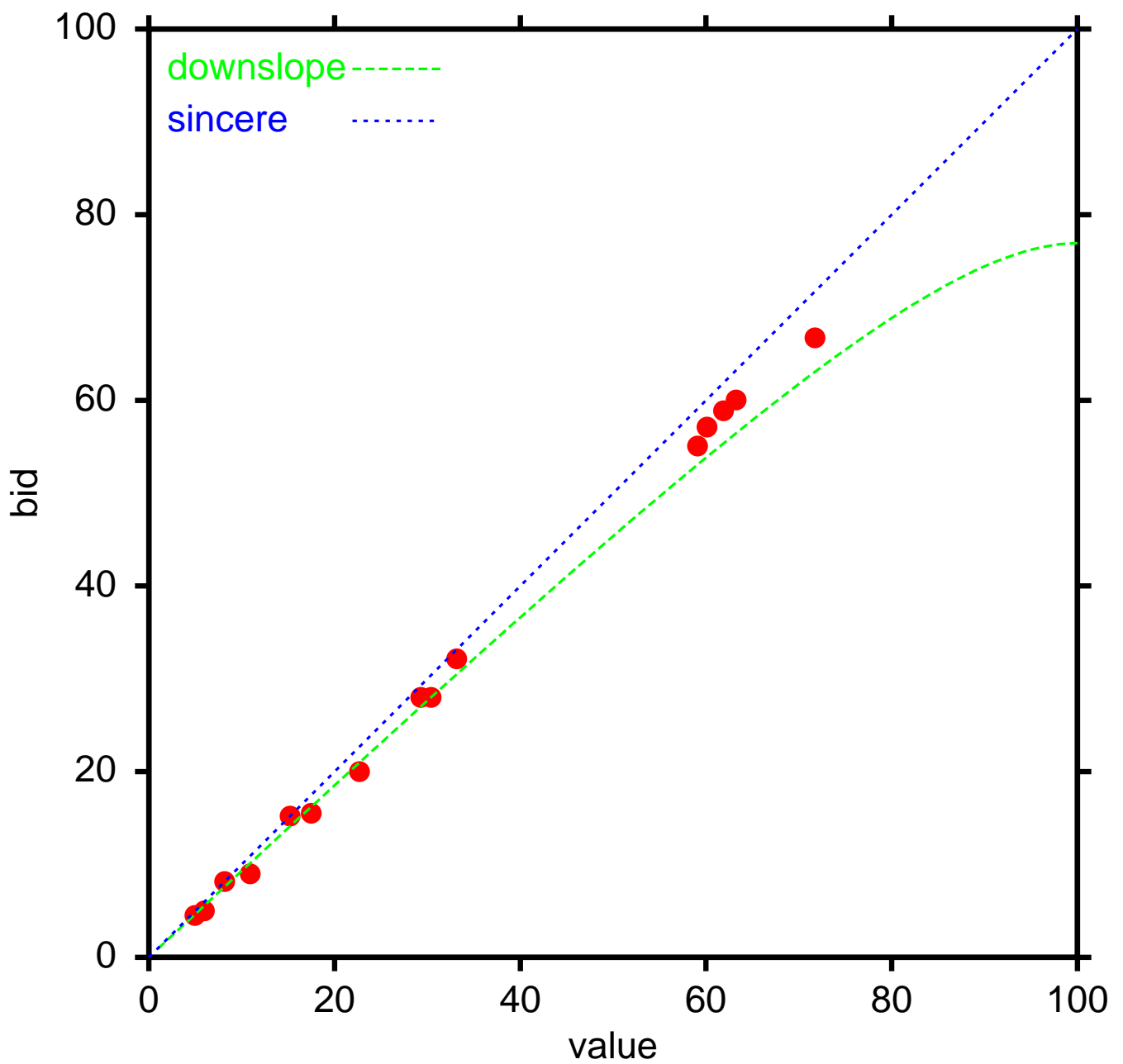
Nash Equilibrium, density is linear downslope [0,100], n=15
