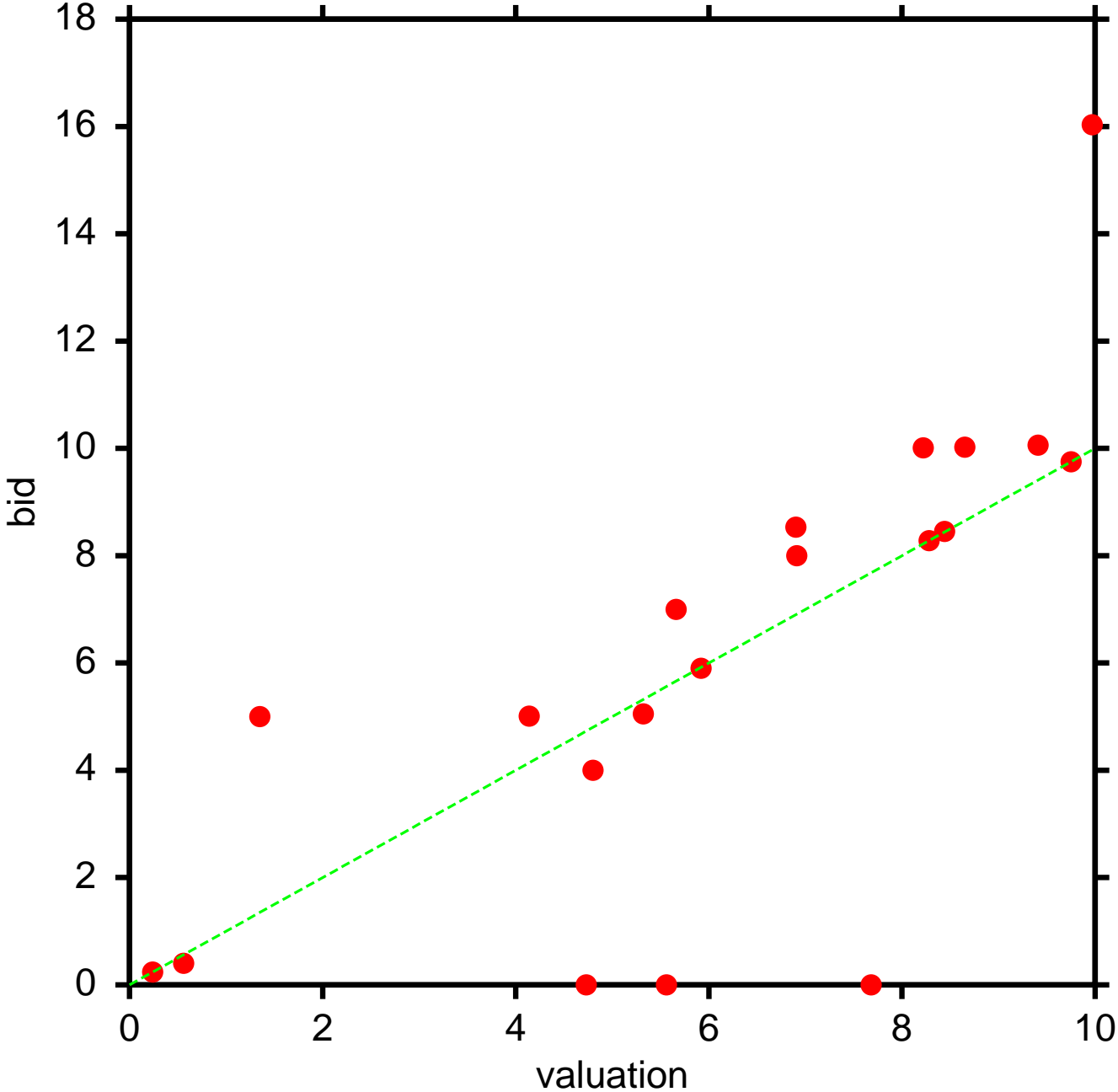
Average-of-Others, sealed-bid, v's iid on [0,$10], Feb. 14, 2008
