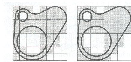
Uniform Voxels
