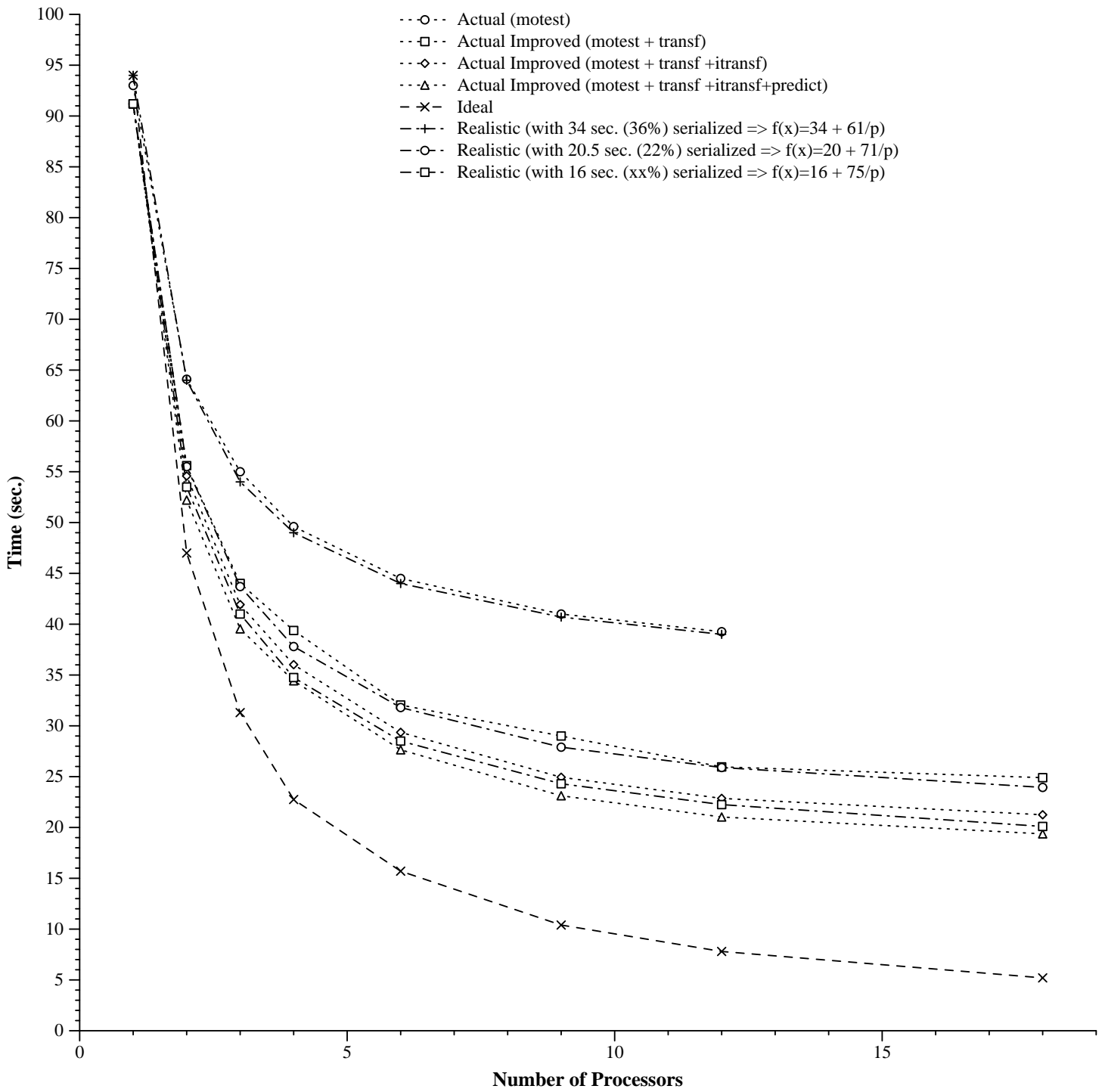
MPEG-2 encoder (46 frames : 720x576 : 36 rows) on toofan.princeton.edu
