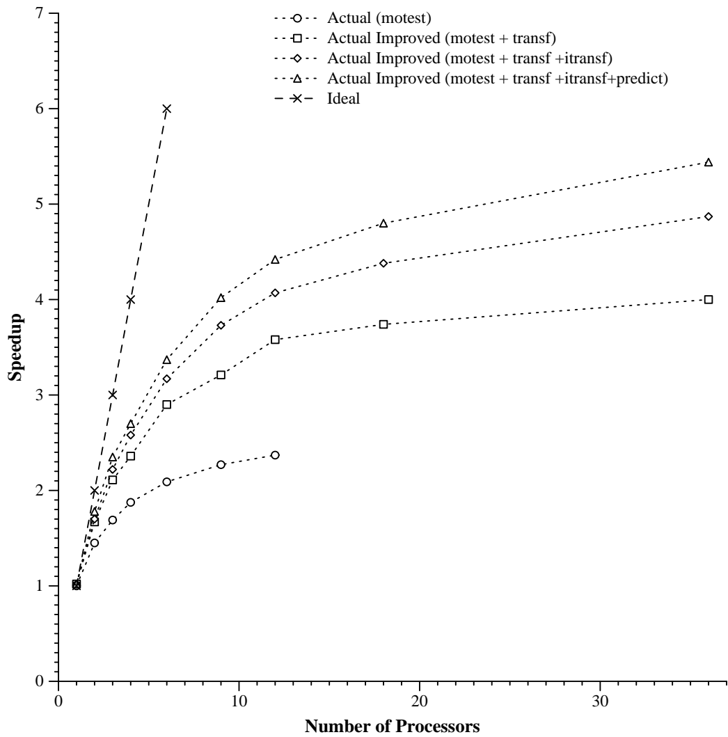
MPEG-2 encoder (46 frames : 720x576 : 36 rows) on toofan.princeton.edu
