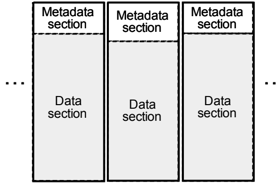
Figure 2: Containers are self-describing, immutable, units of storage several megabytes in size. All segments are stored in containers.
